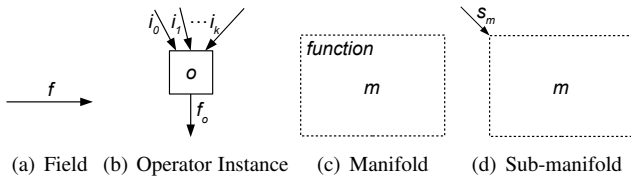
Fig. 1. Proto programs contain manifolds (spaces), fields that assign values to every point in a manifold and operator instances that compute fields.
